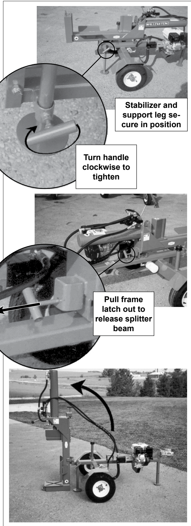
Fig. 14 VERTICAL SPLITTING
