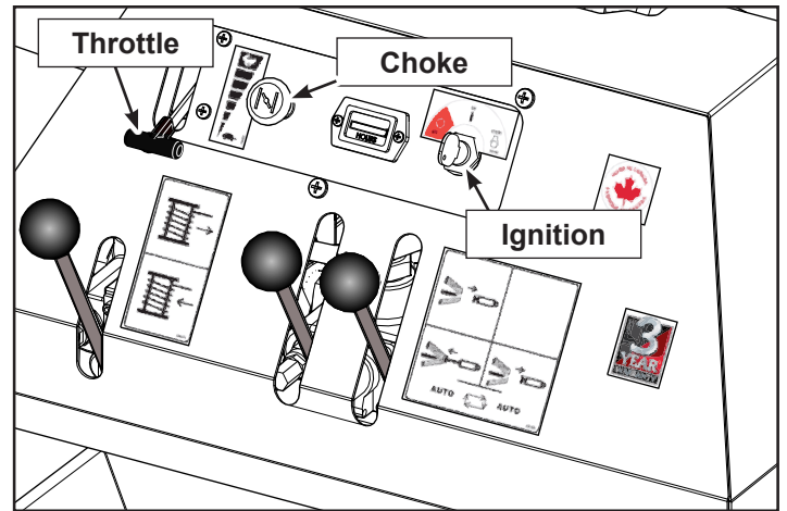
Fig. 17 ENGINE CONTROLS: WP830 & WP860
