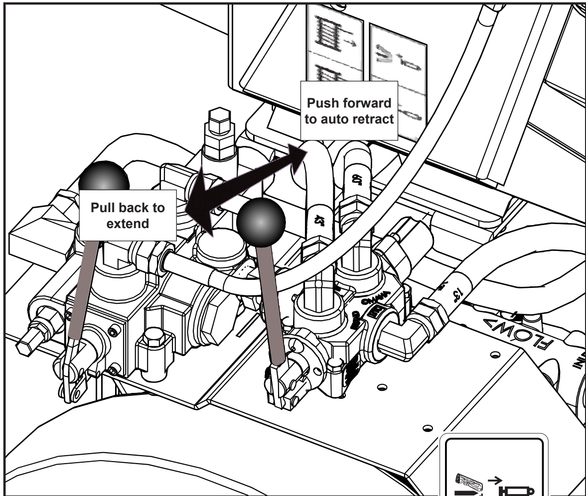
Fig. 8 WP630 SPLITTER CYLINDER CONTROL & LABEL
