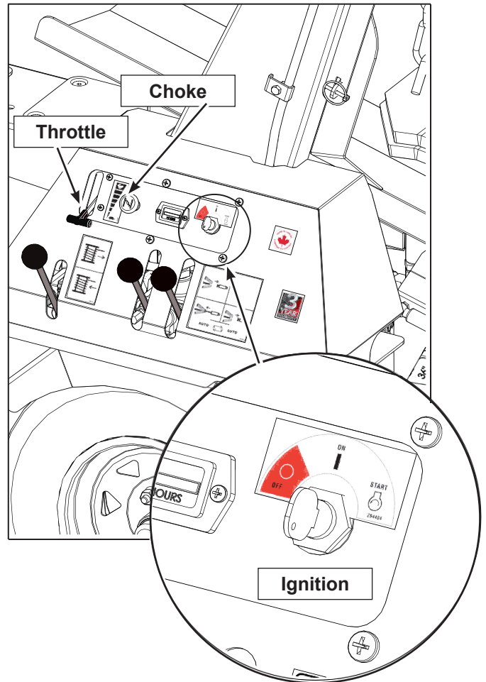
Fig. 2 CONTROLS: WP830 & WP860
