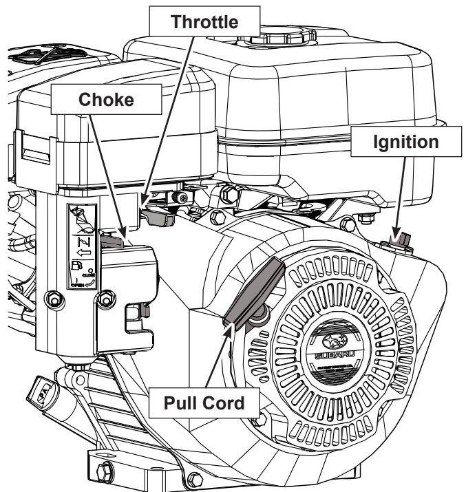
Fig. 18 ENGINE CONTROLS: WP630
