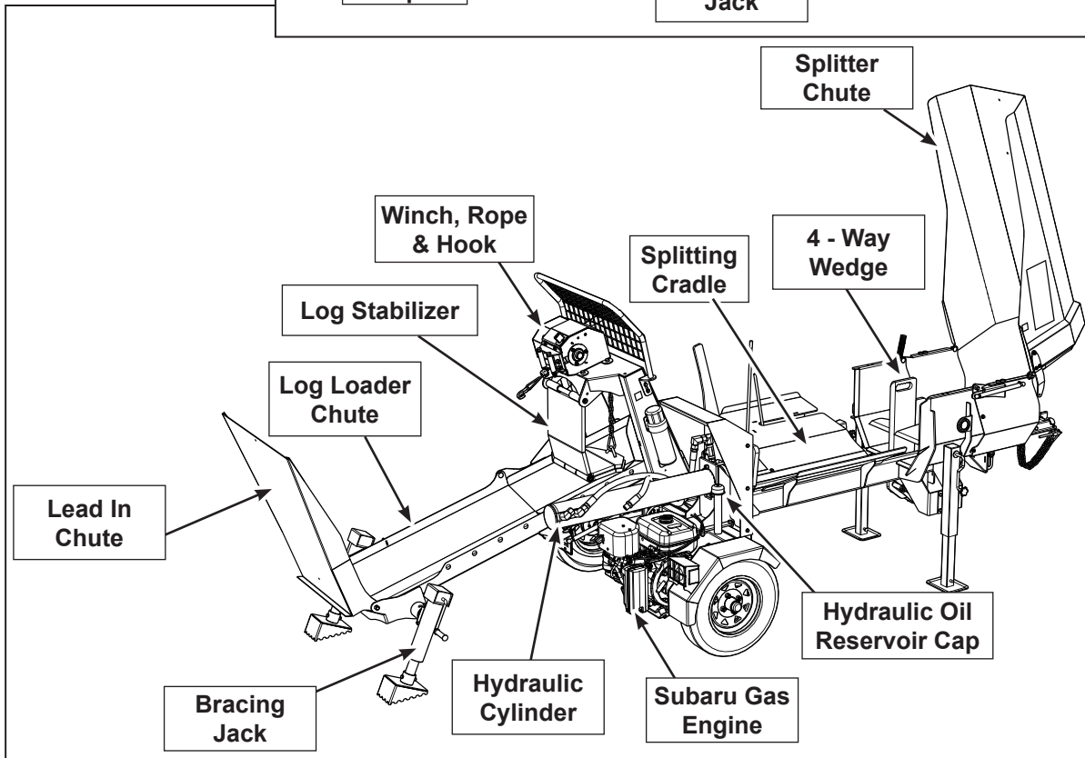
Fig. 1 PRINCIPLE COMPONENTS
