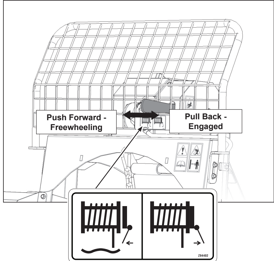
Fig. 6 WINCH GEAR LEVER & LABEL
