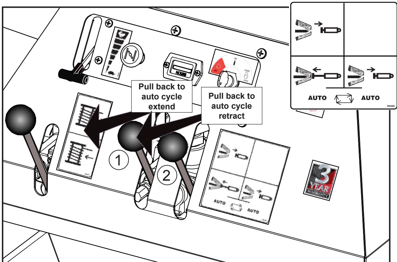
Fig. 7 WP830 and WP860 SPLITTER CYLINDER CONTROL & LABEL
