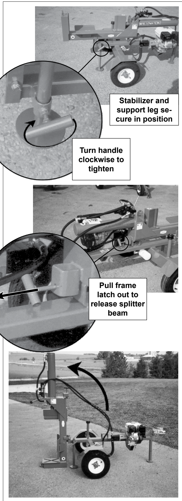
Fig. 14 VERTICAL SPLITTING
