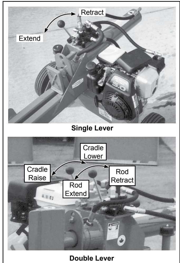
Fig. 8 HYDRAULIC CONTROLS
