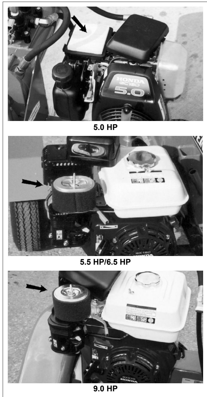
Fig. 22 AIR CLEANER
