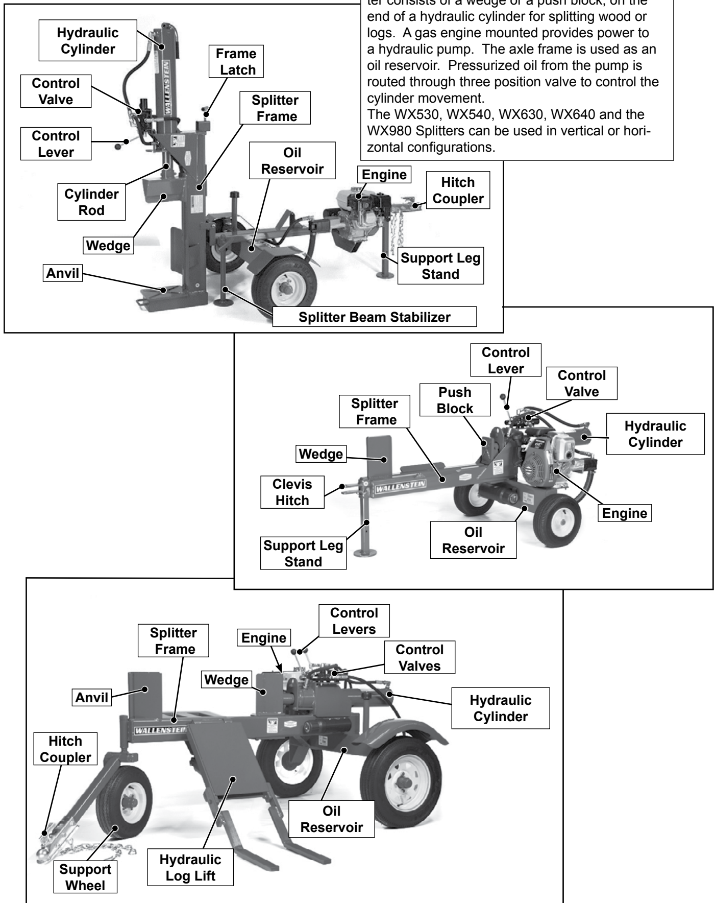
Fig. 1 MACHINE COMPONENTS
