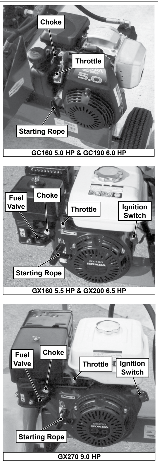
Fig. 7 ENGINE CONTROLS
