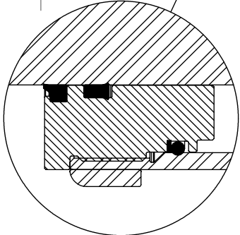
VIEW SHOWS PROPER SEAL ORIENTATION
