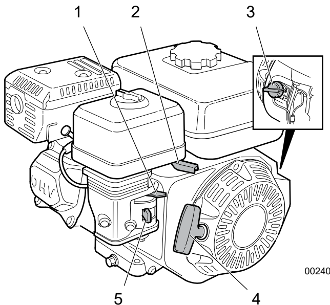
Fig. 7—Engine Controls
