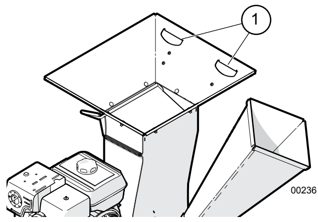
Fig. 27 –Shredder Hopper Handholds
