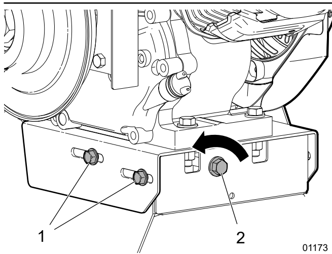
Fig. 37 —Engine Mount
