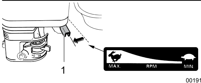
Fig. 11–Engine Throttle Control
