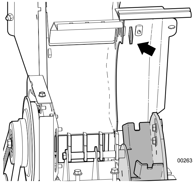
Fig. 53 – Twig Breaker
