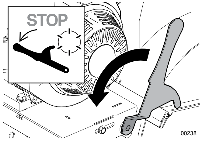
Fig. 16—Disengaging Drive System
