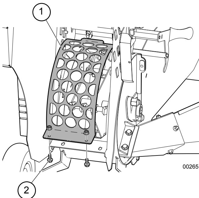
Fig. 54 —Mulching Screen
