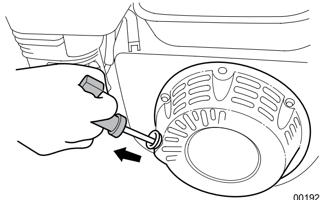
Fig. 23 –Recoil Starter
