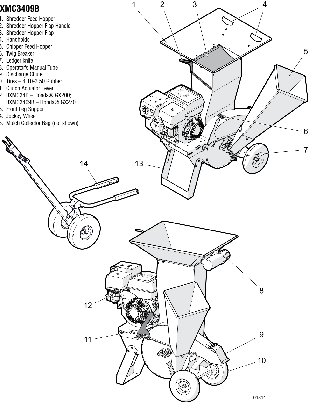
Fig. 3–BXMC34B, BXMC3409B Components
