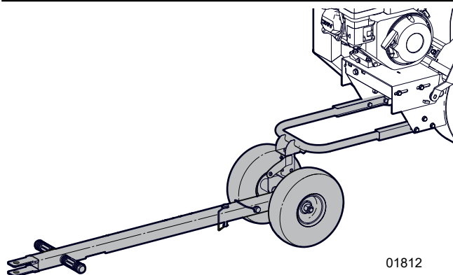
Fig. 34—Jockey Wheel Installation
