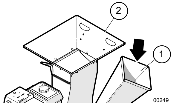
Fig. 25—Chipper Operation
