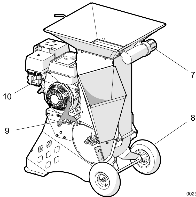
Fig. 5 – BXMC34S, BXMC3409S Components
