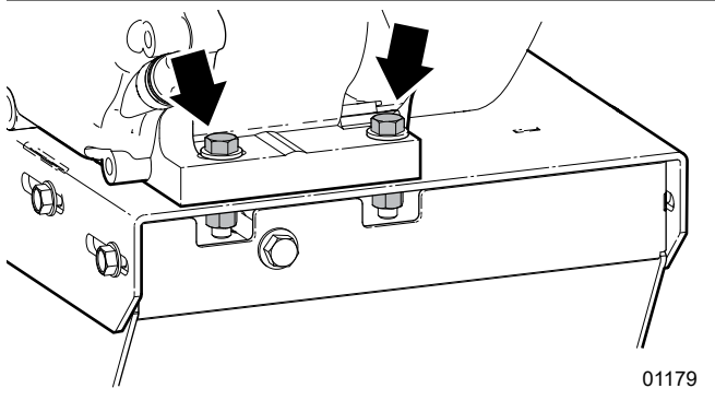
Fig. 43 —Engine bolts
