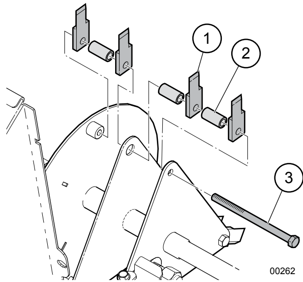
Fig. 51 – Shredder Knives
