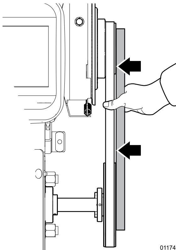
Fig. 41—Sheave Alignment
